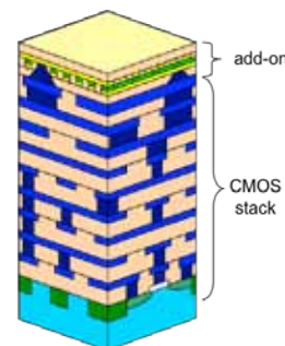
Illustration of 3D hybrid circuit: CMOS subsystem + nano-RRAM add-on
